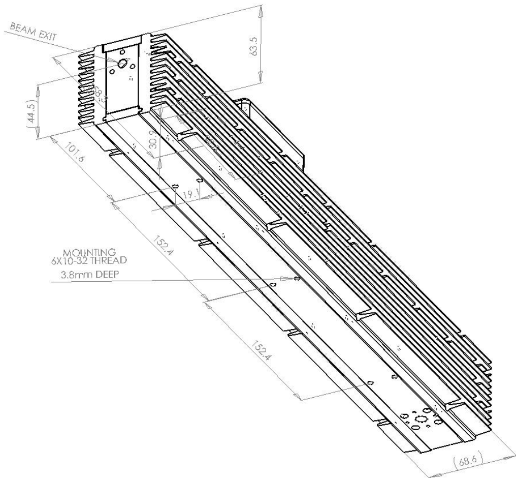
L15 Mounting Illustration, Bottom View, Units in mm
